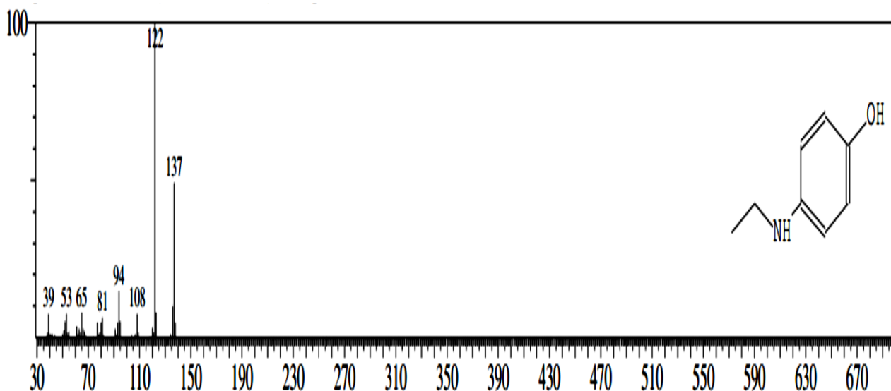
Fig.(2): Chemical structure and GC –Mass spectroscopy of compound Phenol, 4-(ethylamino)- 4-Ethylaminophenol.
