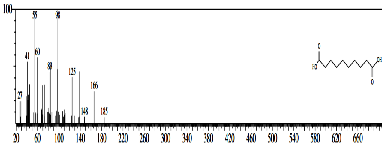
Fig.(1): Chemical structure and GC –Mass spectroscopy of compound 1,10-Decanedioic acid.
