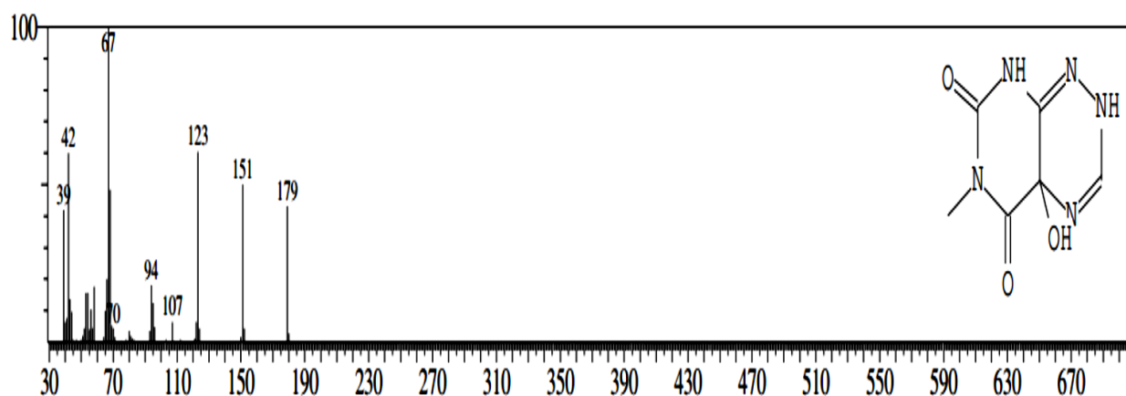
Fig.(3): Chemical structure and GC –Mass spectroscopy of compound Pyrimido[5,4-E]-1,2,4-triazine-5,7(4ah,6H)-dione, 8,8a-dihydro-4a-hydroxy-6-methyl.
